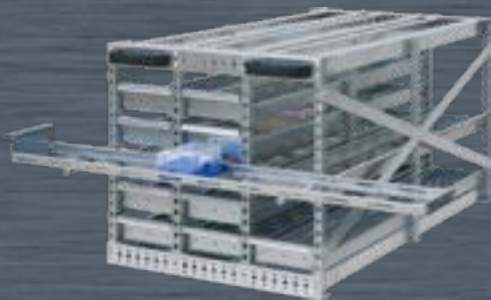
Optional drawer system for the storage of pharmaceutical products under deep-freeze conditions
