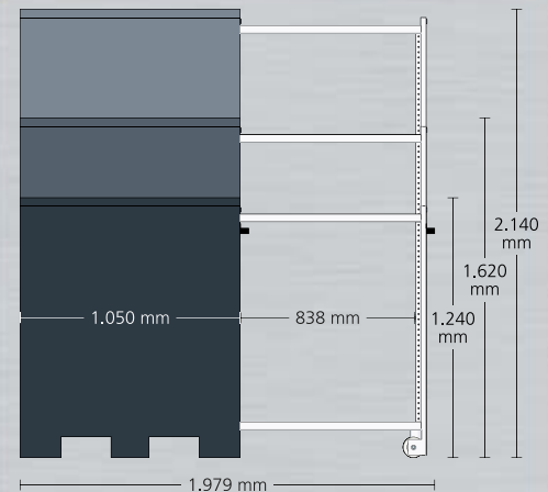
660 width WKS 013 1,050 depth WKS 033 1,300 depth
